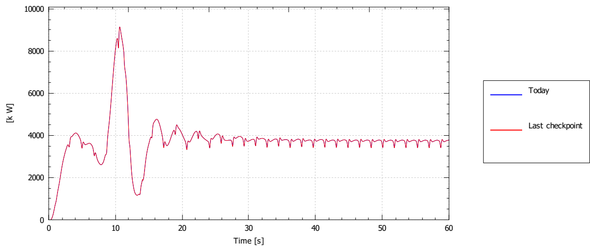
Power (aero)
